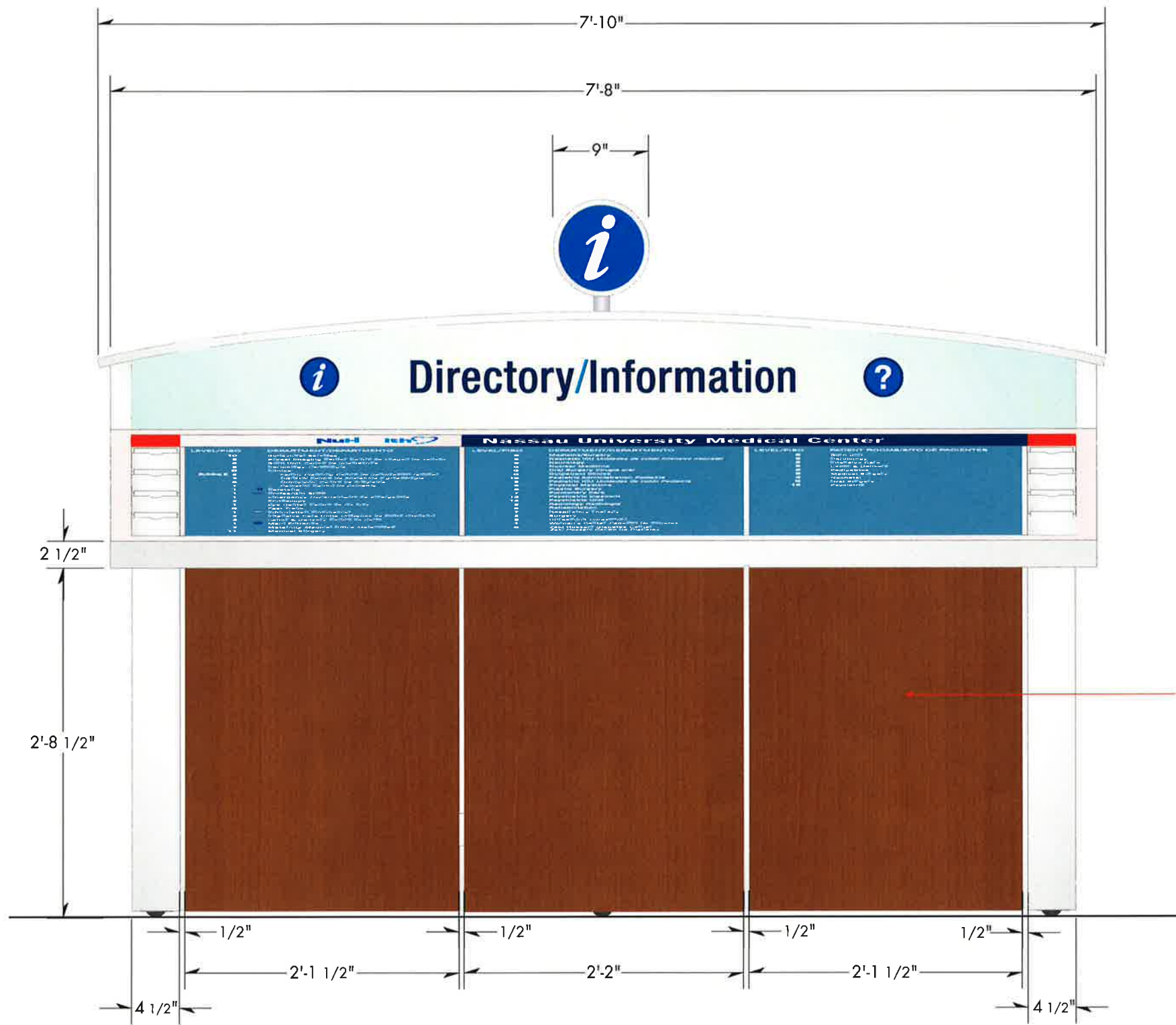
A Information Directory freestanding in main entry (Carman Avenue) corridor/Level 1 typical Scale: 1" = 1'-0"
