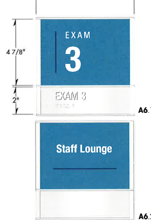
A6 Primary Room ID Standard ClearPath™ extrusion with NEW top cap, printed insert and separate Braille/tactile insert by fabricator A6.1 Qty: 103 (one hundred and three) A6.2 Qty: 17 (seventeen)
