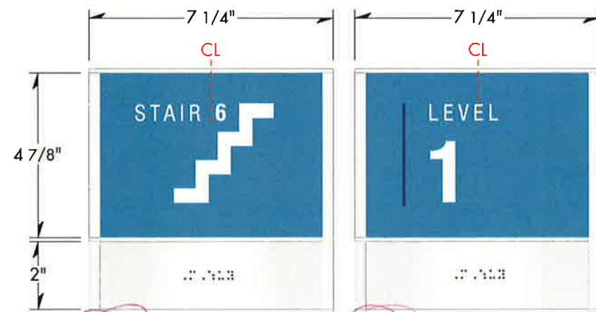
A8 Primary Room Standard ClearPath™ extrusion with NEW top cap, printed insert and separate Braille/tactile insert by fabricator A8.1 Qty: 22 (twenty-two) A8.2 Qty: 23 (twenty-three)
