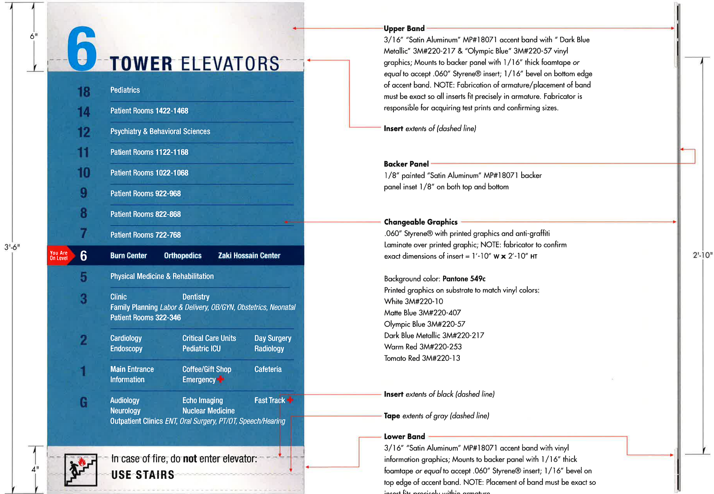
E3 1 Elevator Directory single panel Level 6 Scale: 1:5
