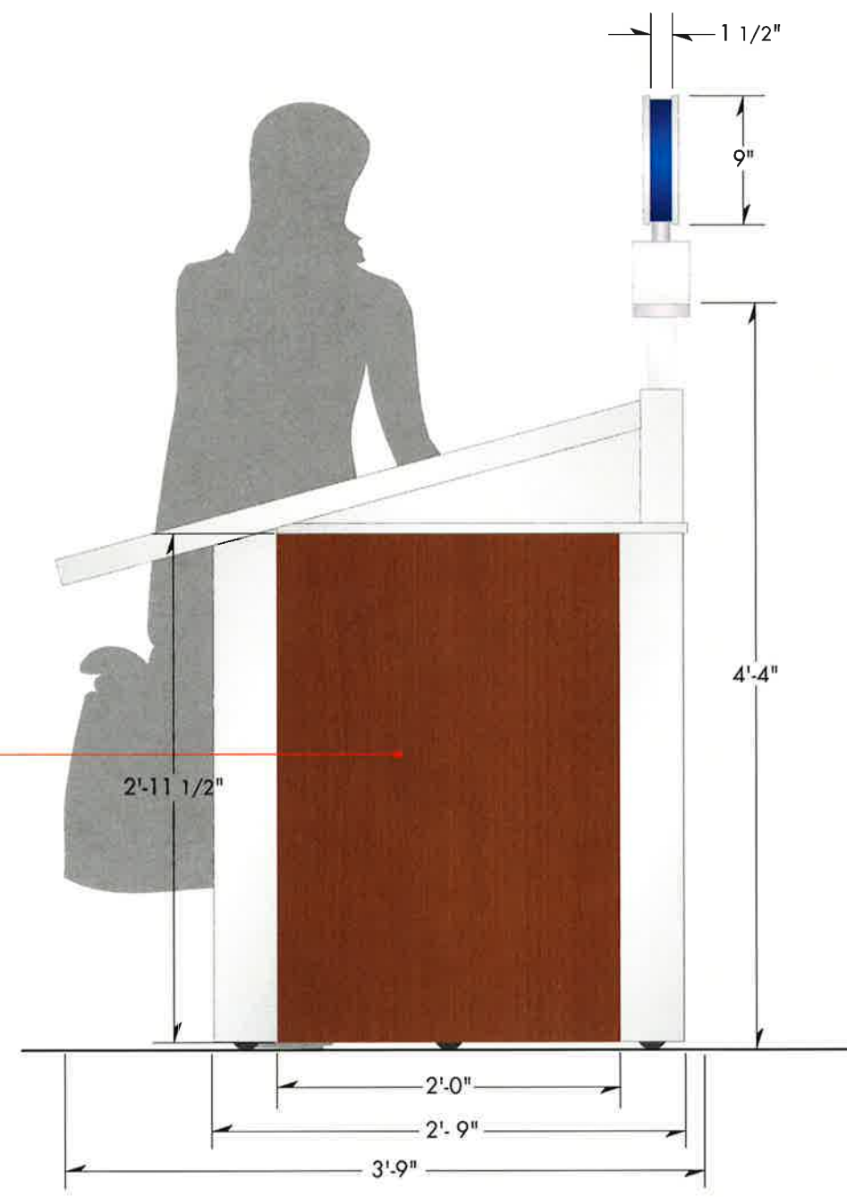
B Information Directory Side Elevation typical Scale: 1" = 1'-0"
