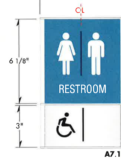
A7.1 Restroom ID door-mounted Standard ClearPath™ extrusion with NEW top cap and printed insert by fabricator Qty: 44 (fourty-four)
