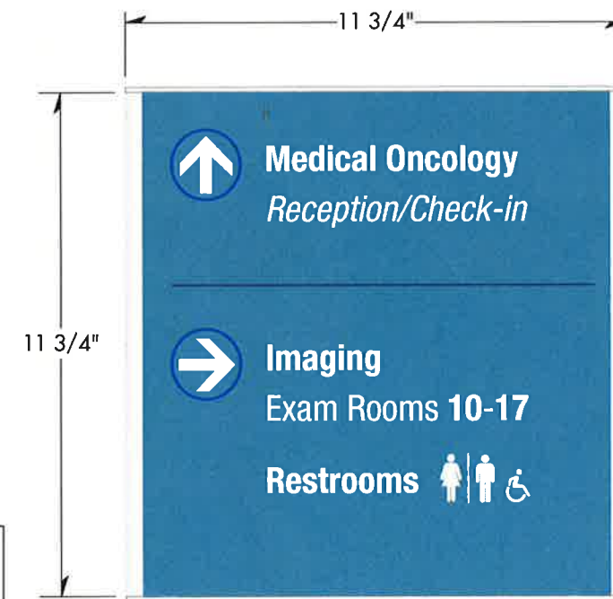
D4 Tertiary Directional Standard ClearPath™ extrusion w/NEW top cap & printed insert by fabricator Qty: 0 (zero)
