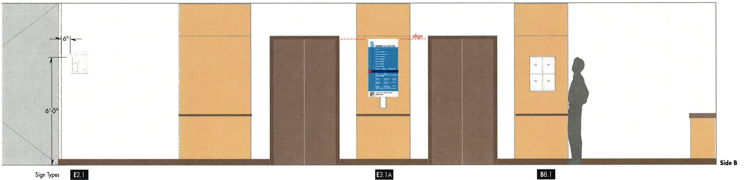
A Elevator Sign Placement wall mounted signs Level 5 - typical (Levels 2-19) Scale: 1/4" = 1'-0"
