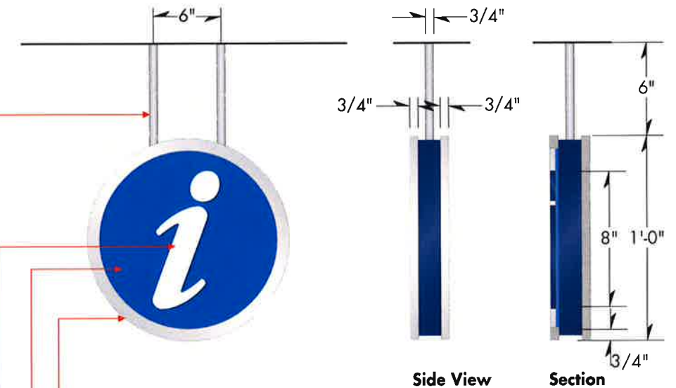
Side View
