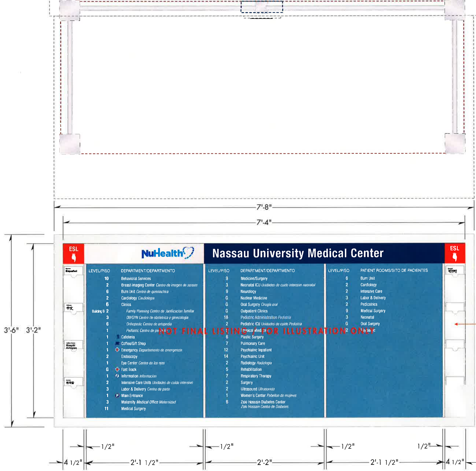
C Information Directory digitally printed graphic panel inserts Scale: 1" = 1'-0"
