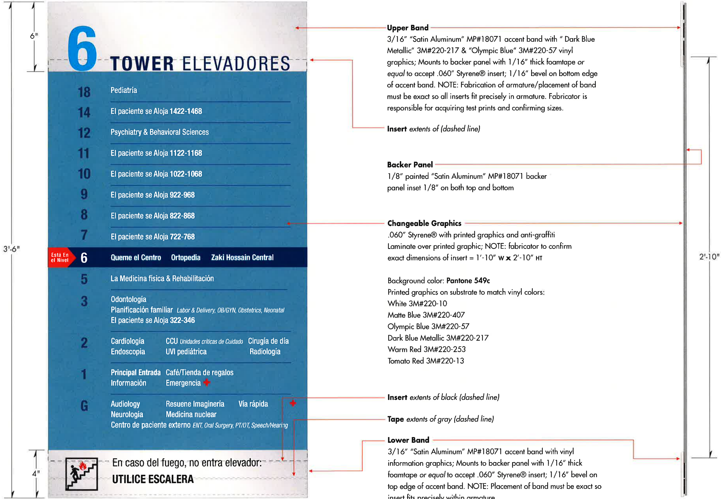
E3 Elevator Directory single panel Level 6 1 Scale: 1:5
